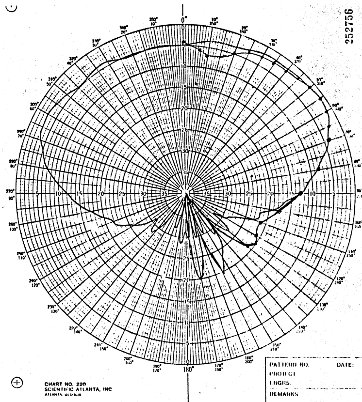
Fig. 12 - Crossed dipoles theoretical and measured radiation patterns for RHCP polarization.
