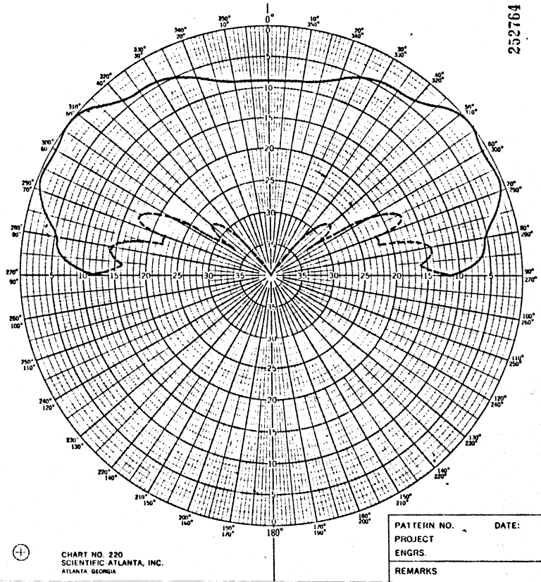
Fig. 9 - Quadrifilar antenna radiation pattern. Antenna above an infinite ground plane. h = 0.05 \text{ m} , N = 3 , R_0 = 0.0125 \text{ m} , L_{ax} = 0.2298 \text{ m} , P = 0.2298 \text{ m} . ——— RHCP - - - - LHCP
