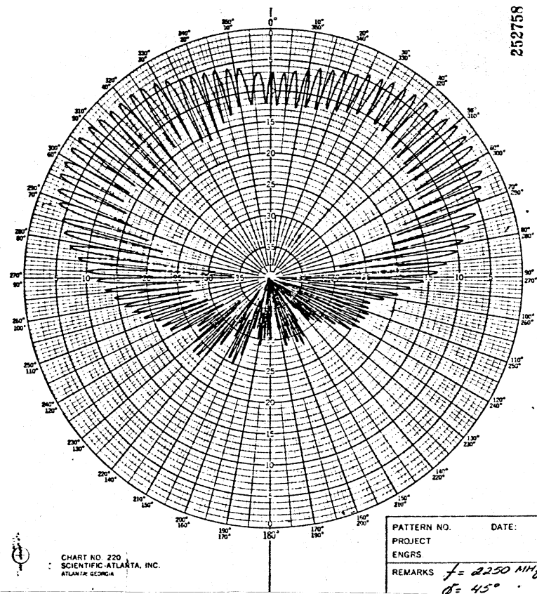
Fig. 14 - Crossed dipoles radiation pattern, Rotating Source.
